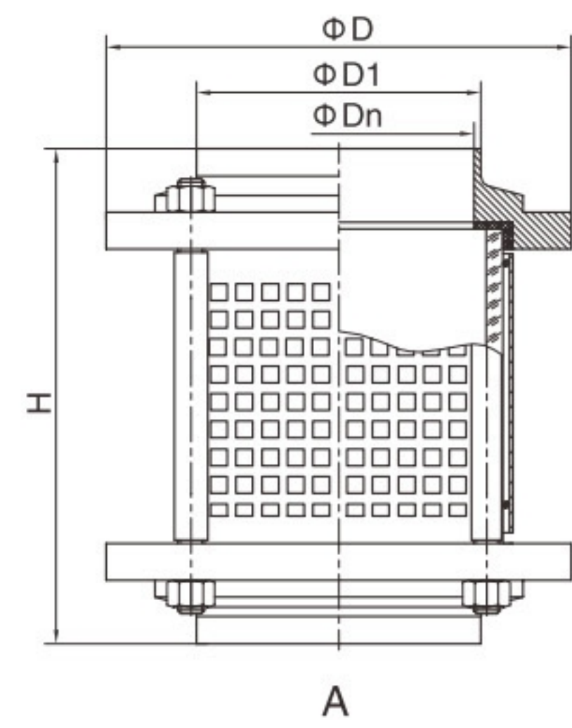
焊接直通视镜(DIN) Welded Straight Sight Glass
