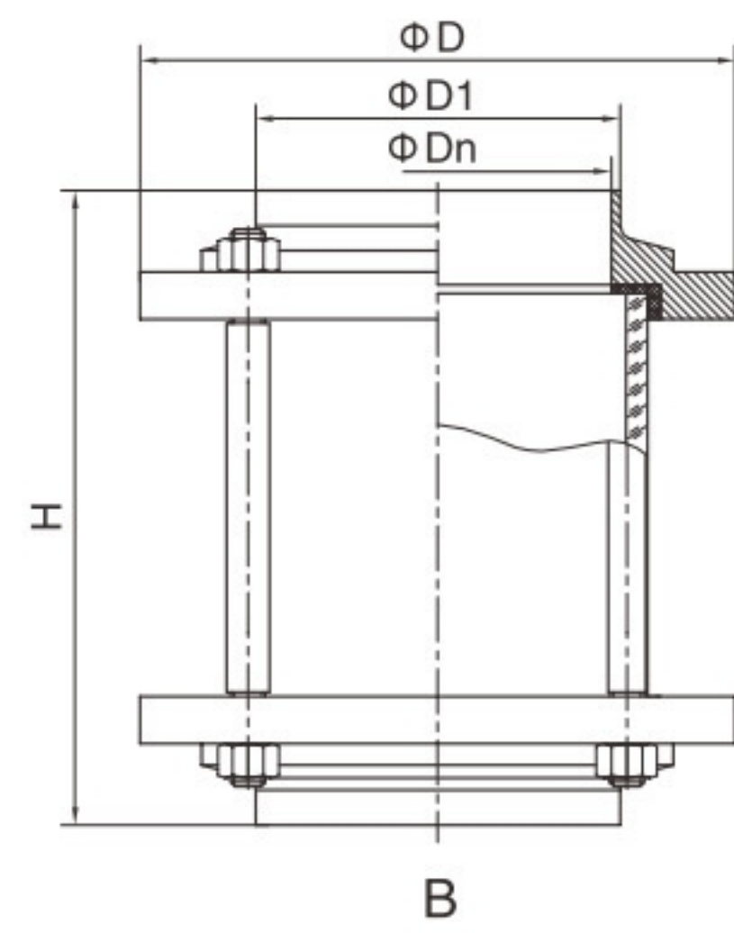
焊接直通视镜(3A) Welded Straight Sight Glass
