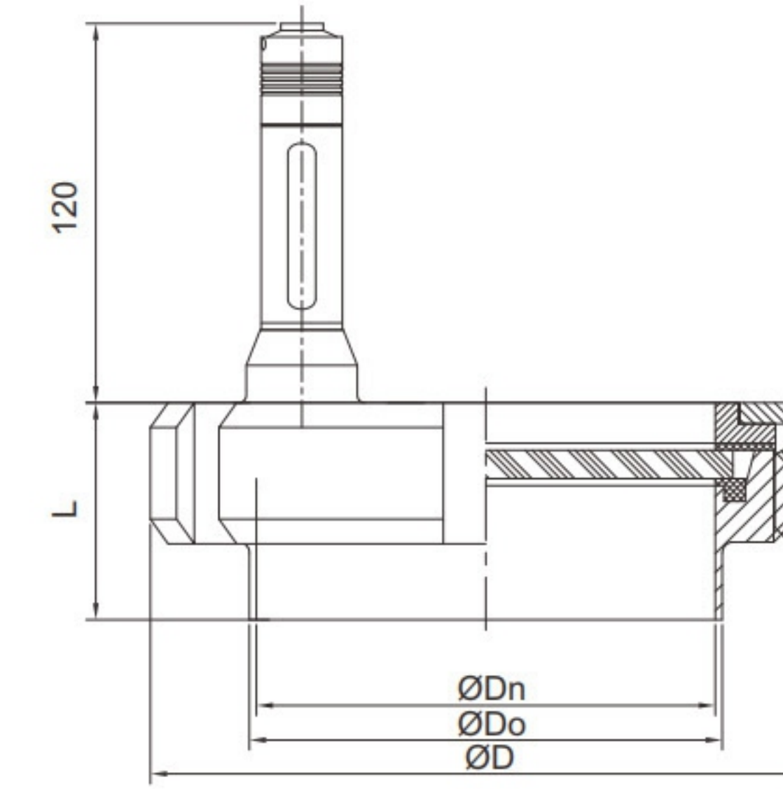
Stainless steel Luminaire Sight Glass
