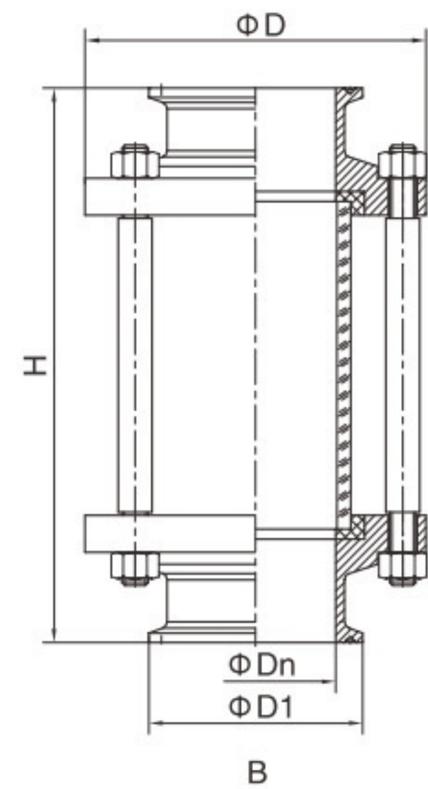
快装直通视镜(3A) Clamped Straight Sight Glass
